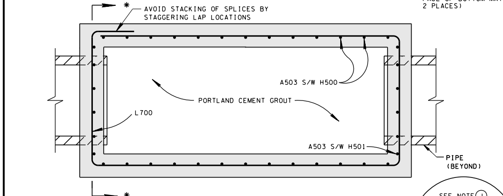
SECTION E-E
